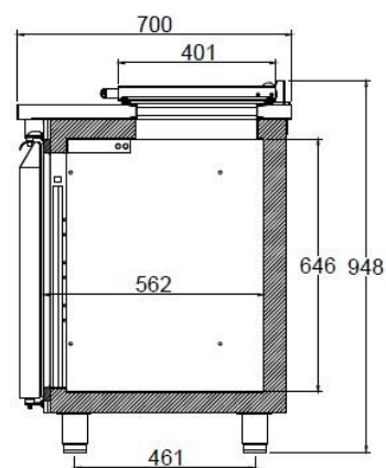
SECTION B-B
